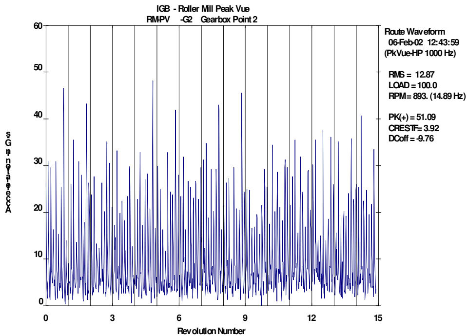
Figure 1 PeakVue time waveform on input shaft to roller mill gearbox at 890 RPM
