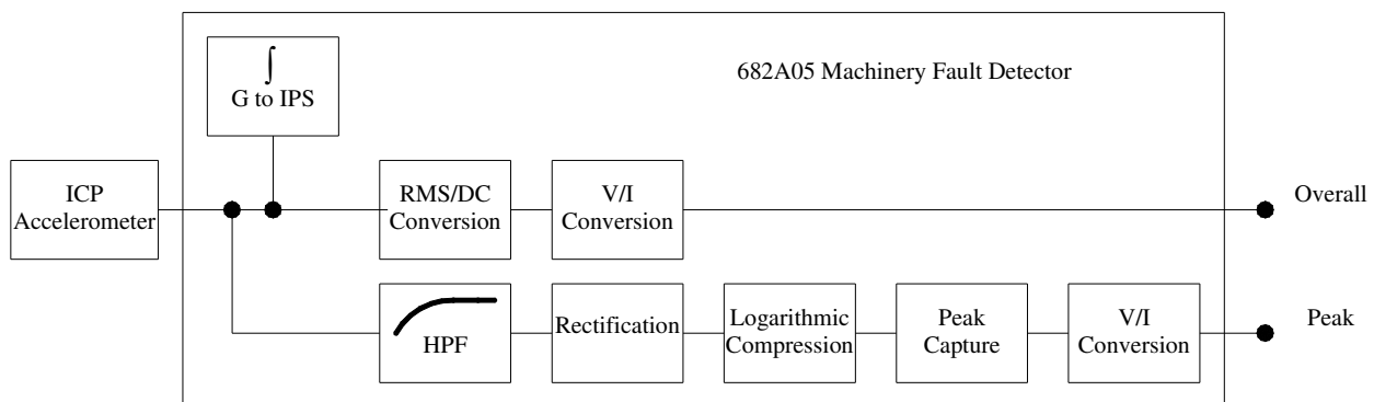
Flow Diagram 1
